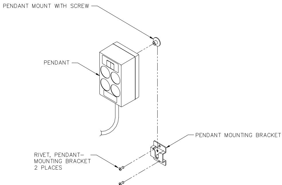
FIG.1: PENDANT MOUNTING DIAGRAM
