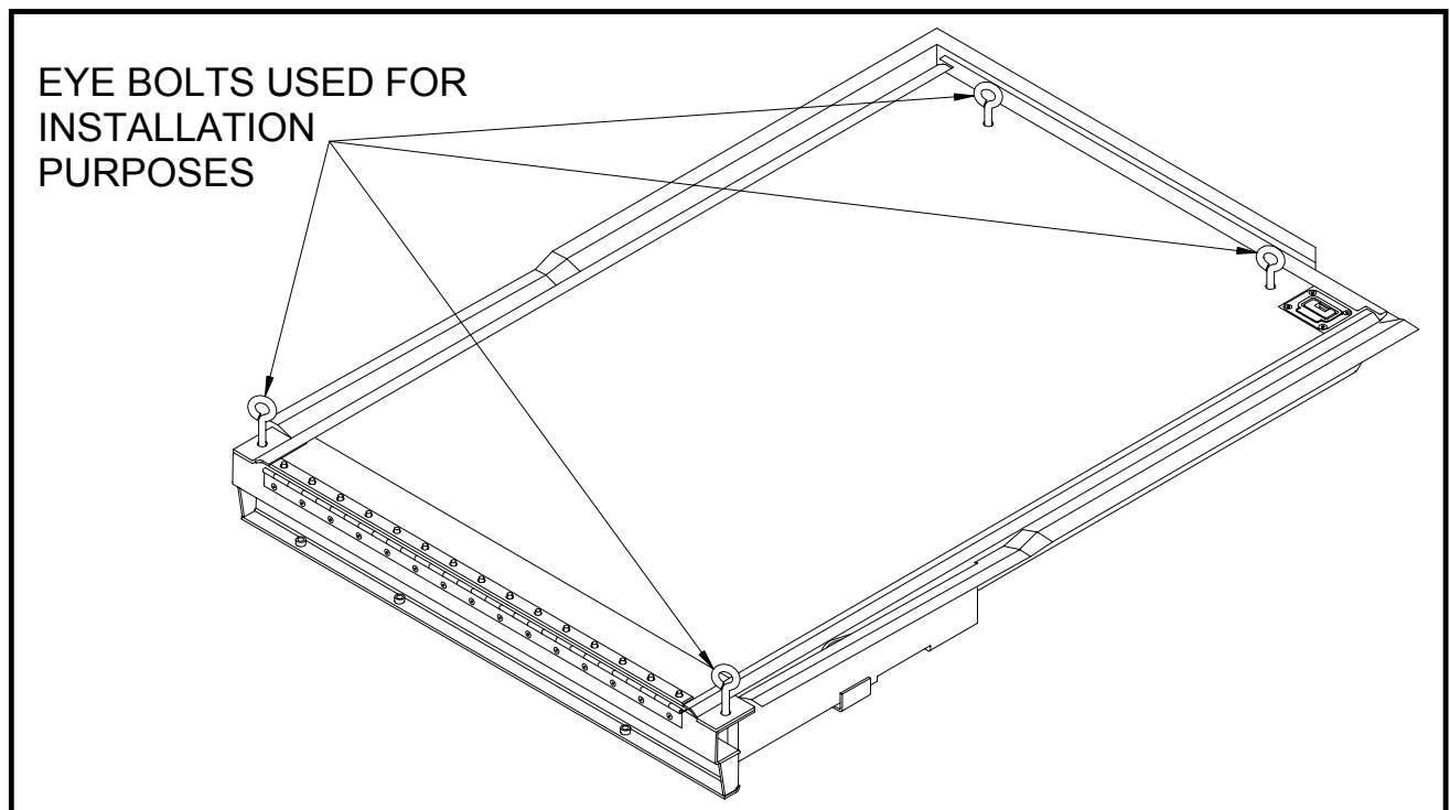
FIG [1]: IDENTIFICATION OF (4) EYE BOLTS FOR INSTALLATION PURPOSES (AS SHIPPED).
