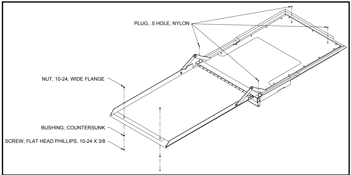
FIG [2]: PLUG AND HARDWARE LOCATION (S)
