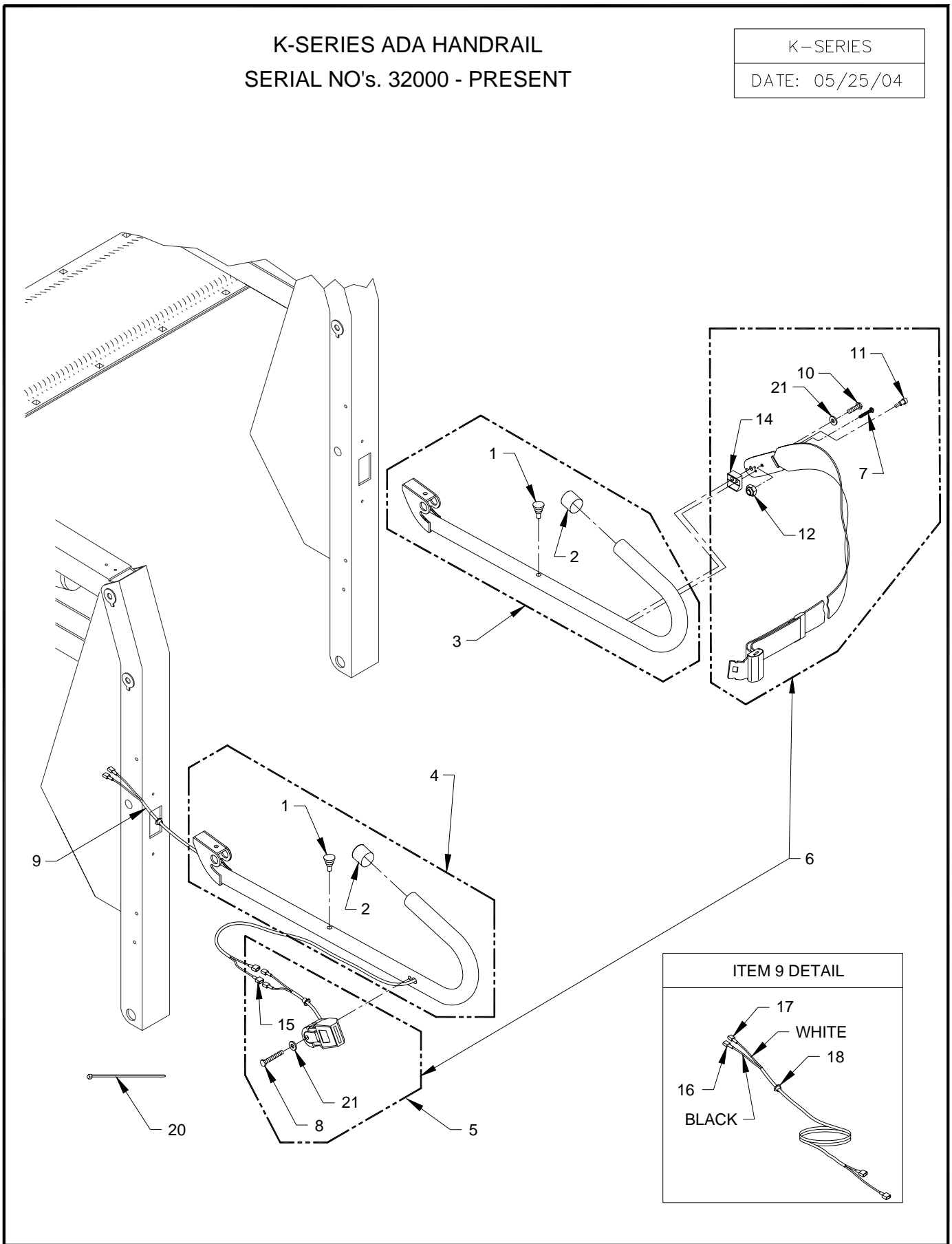
FIGURE 4-15: ADA HANDRAIL ASSEMBLIES
